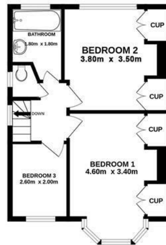
1ST FLOOR 433 sq.ft. (40.2 sq.m.) approx.
